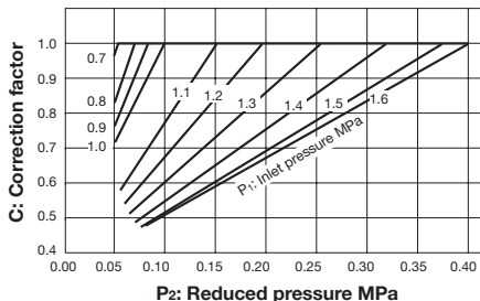
Fig. 1: Corrected Cv value
